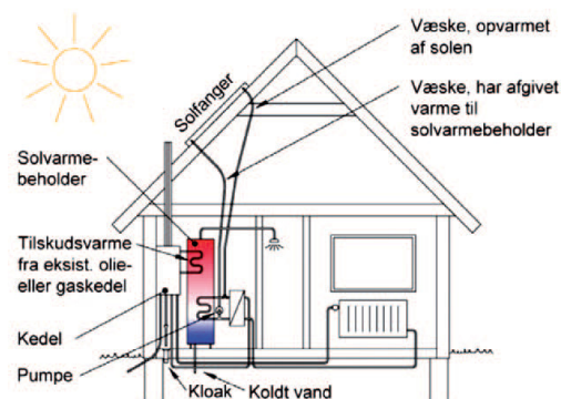
Figure 19: Illustration of a solar thermal heating system 5
